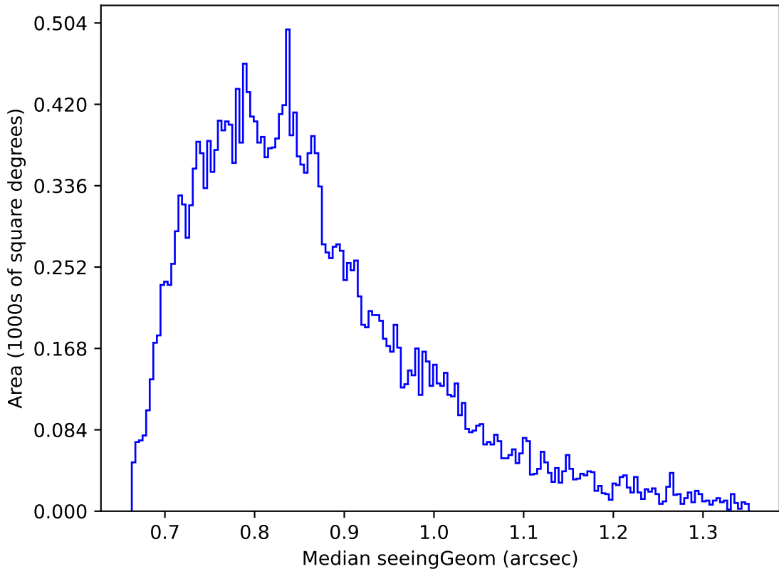
ddf_loaded_fl1_v3.4_10yrs Yr 1 r band: Median seeingGeom
