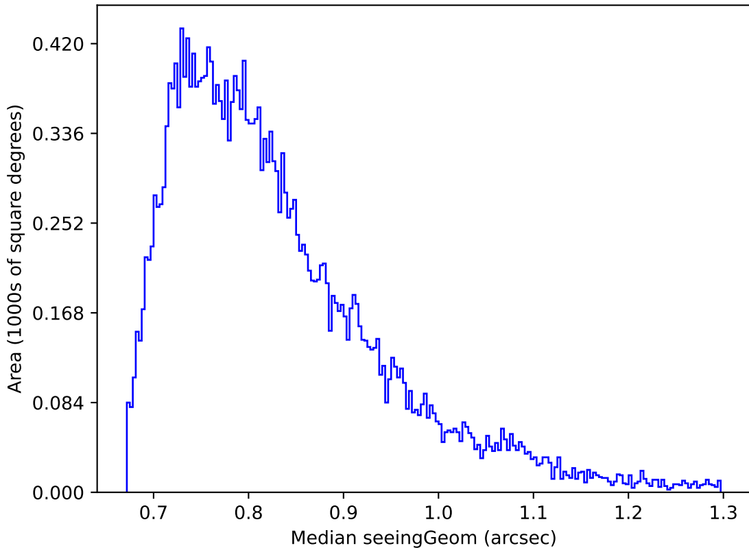
ddf_loaded_fl1_v3.4_10yrs Yr 1 i band: Median seeingGeom
