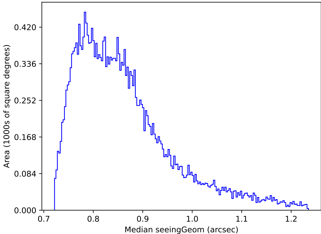
ddf_loaded_fl1_v3.4_10yrs Yr 1 all bands: Median seeingGeom
