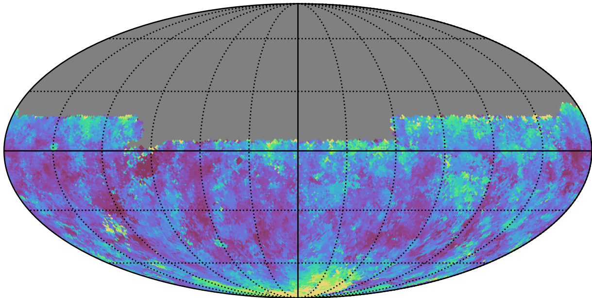
ddf_loaded_fl1_v3.4_10yrs Yr 1 y band: Median seeingEff
