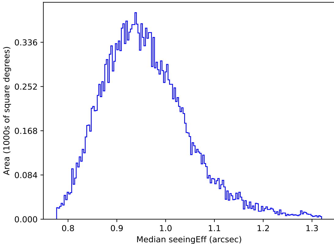
ddf_loaded_fl1_v3.4_10yrs Yr 1 y band: Median seeingEff
