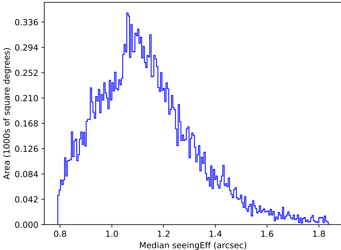
ddf_loaded_fl1_v3.4_10yrs Yr 1 u band: Median seeingEff
