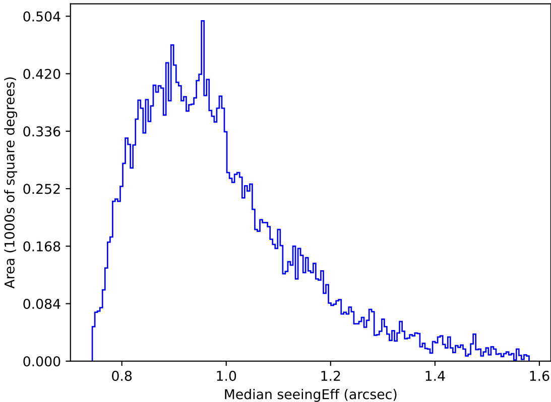
ddf_loaded_fl1_v3.4_10yrs Yr 1 r band: Median seeingEff
