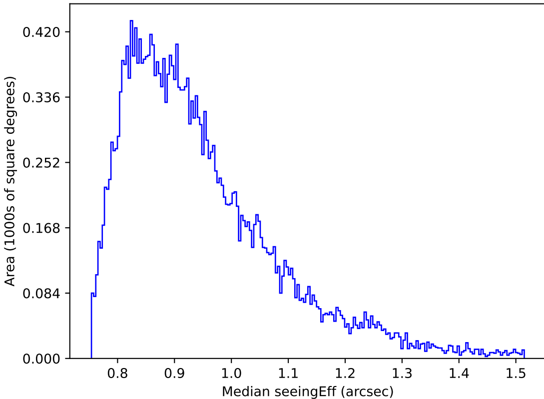
ddf_loaded_fl1_v3.4_10yrs Yr 1 i band: Median seeingEff
