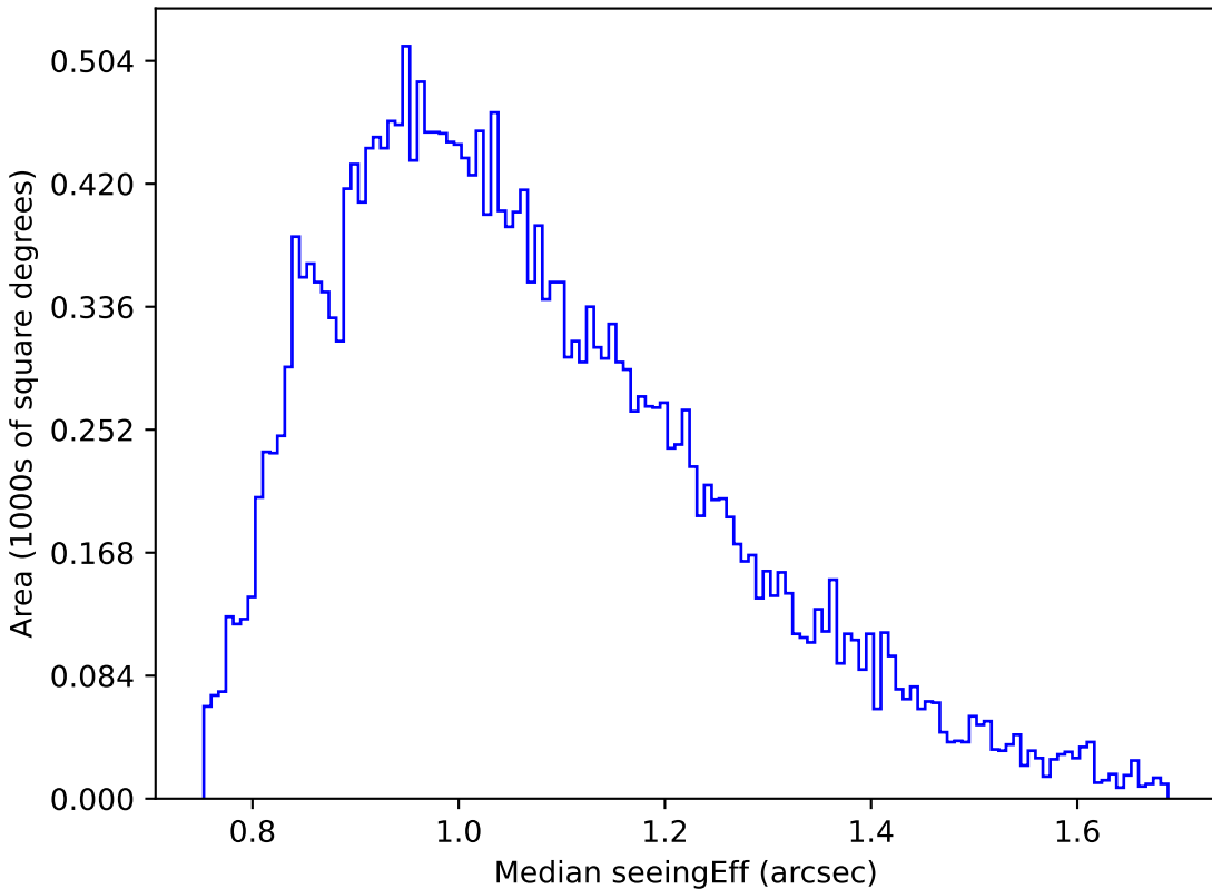
ddf_loaded_fl1_v3.4_10yrs Yr 1 g band: Median seeingEff
