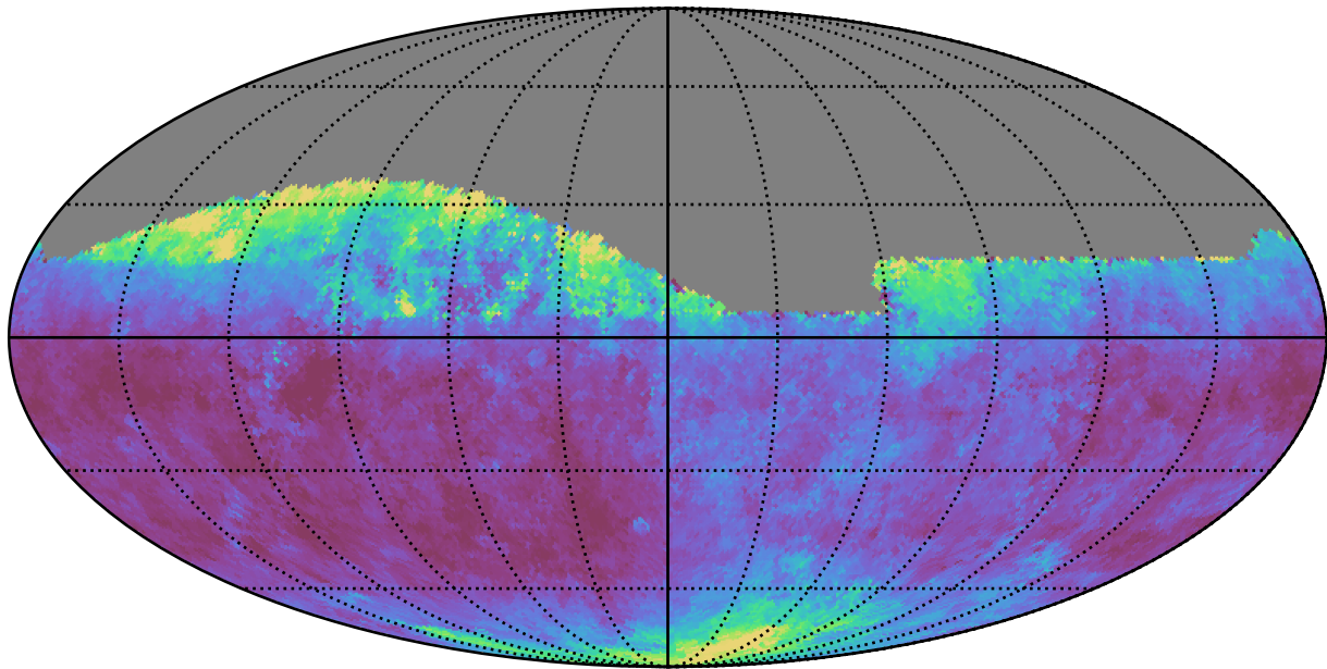
ddf_loaded_fl1_v3.4_10yrs Yr 1 all bands: Median seeingEff
