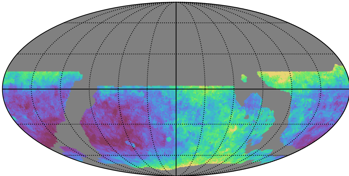
ddf_loaded_fl1_v3.4_10yrs WFD z band: Median seeingEff
