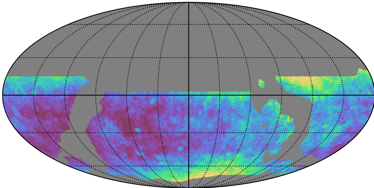
ddf_loaded_fl1_v3.4_10yrs WFD y band: Median seeingEff
