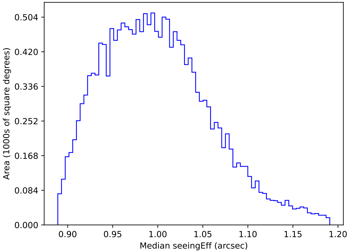
ddf_loaded_fl1_v3.4_10yrs WFD y band: Median seeingEff
