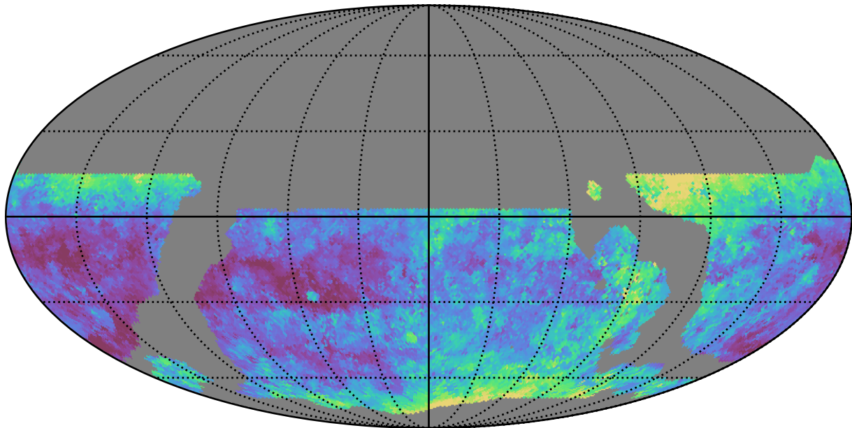
ddf_loaded_fl1_v3.4_10yrs WFD u band: Median seeingEff
