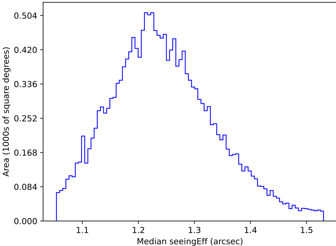
ddf_loaded_fl1_v3.4_10yrs WFD u band: Median seeingEff
