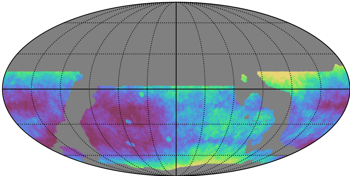
ddf_loaded_fl1_v3.4_10yrs WFD r band: Median seeingEff
