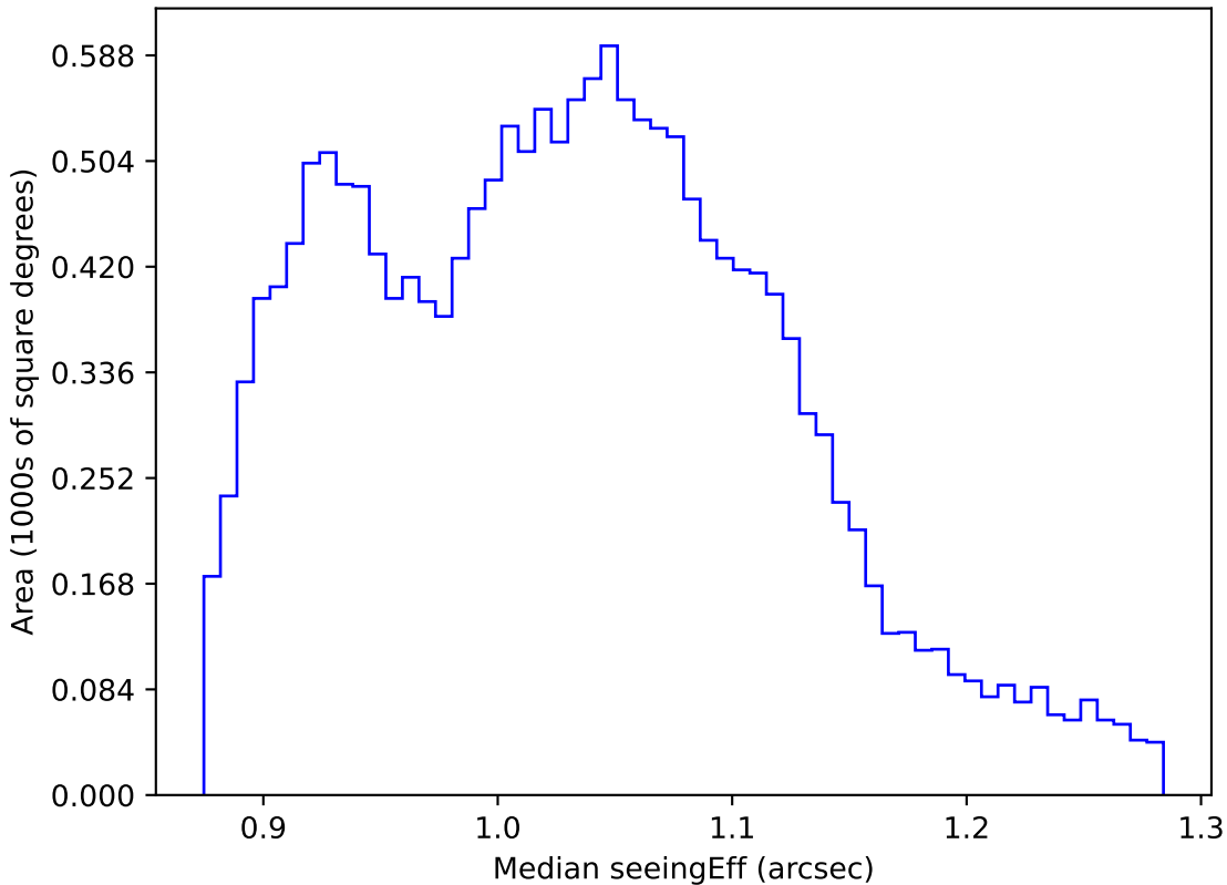
ddf_loaded_fl1_v3.4_10yrs WFD r band: Median seeingEff
