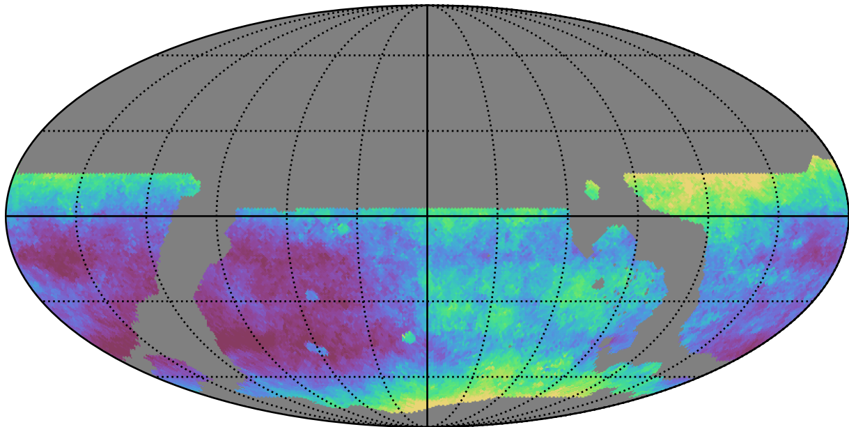
ddf_loaded_fl1_v3.4_10yrs WFD i band: Median seeingEff
