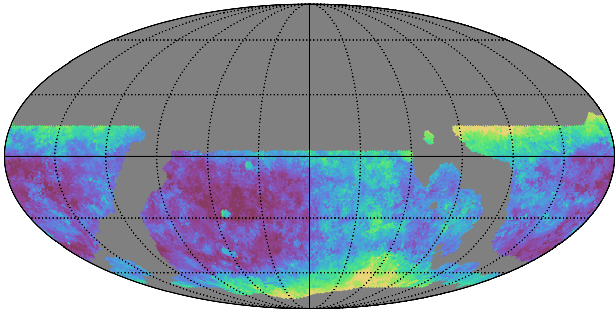
ddf_loaded_fl1_v3.4_10yrs WFD g band: Median seeingEff
