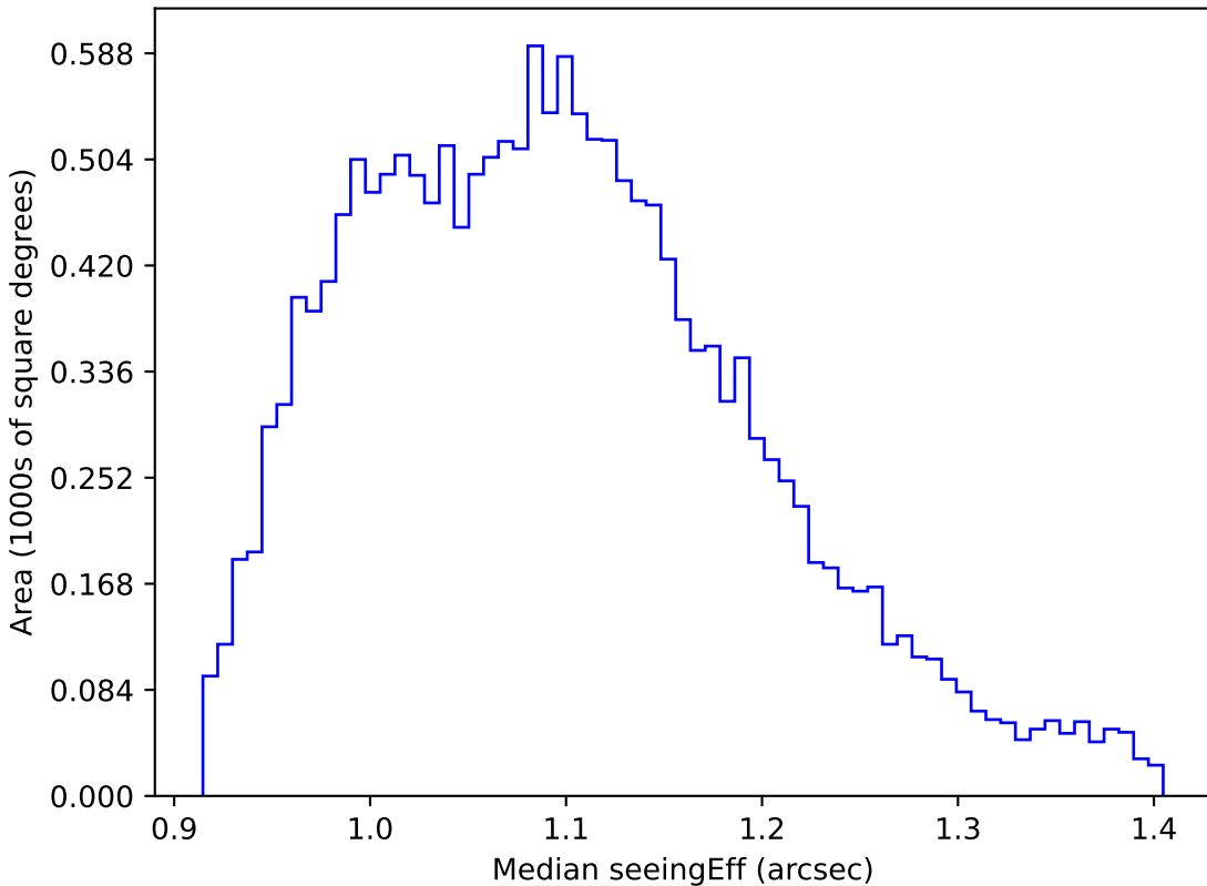
ddf_loaded_fl1_v3.4_10yrs WFD g band: Median seeingEff
