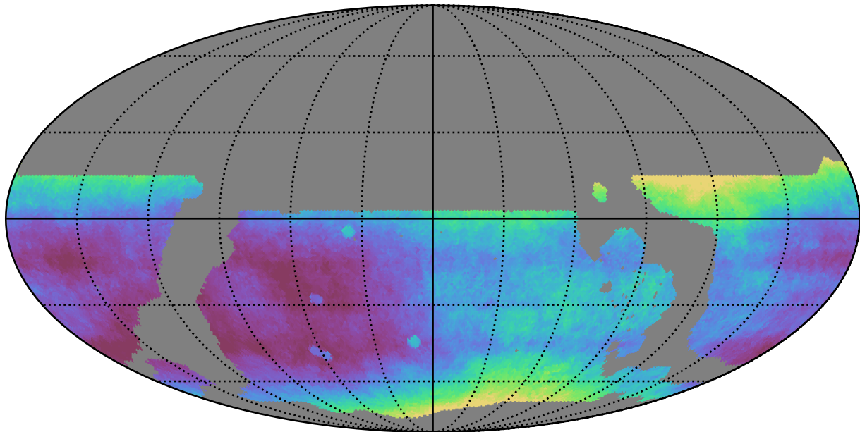
ddf_loaded_fl1_v3.4_10yrs WFD all bands: Median seeingEff
