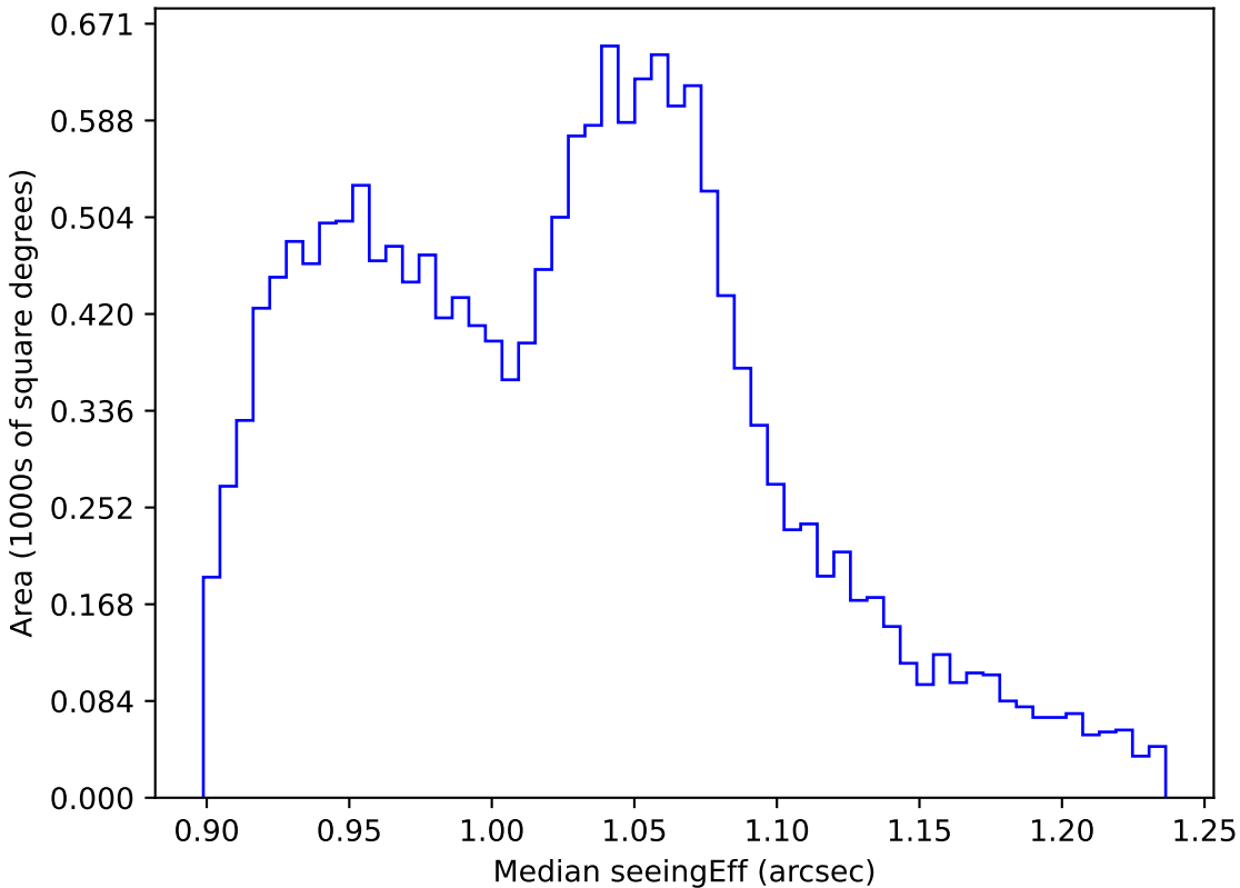
ddf_loaded_fl1_v3.4_10yrs WFD all bands: Median seeingEff
