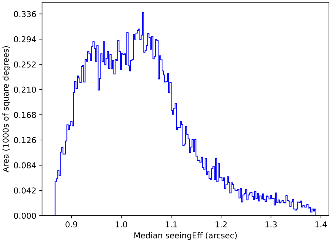
ddf_loaded_fl1_v3.4_10yrs All sky z band: Median seeingEff
