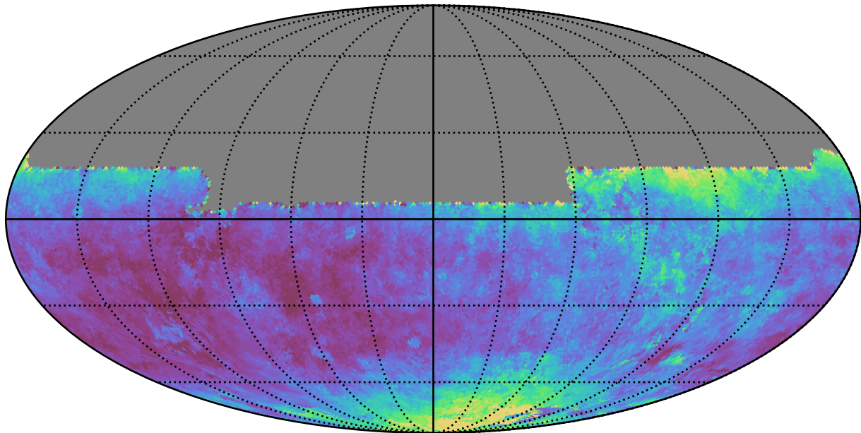
ddf_loaded_fl1_v3.4_10yrs All sky y band: Median seeingEff
