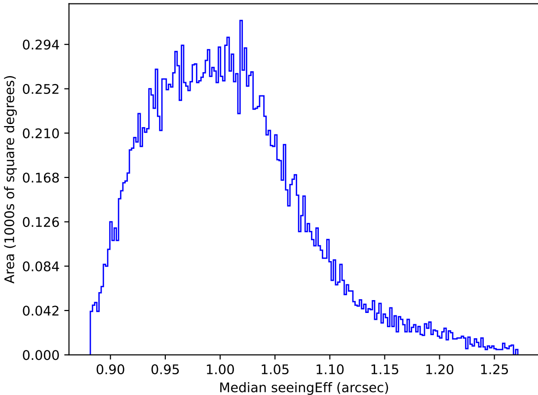
ddf_loaded_fl1_v3.4_10yrs All sky y band: Median seeingEff
