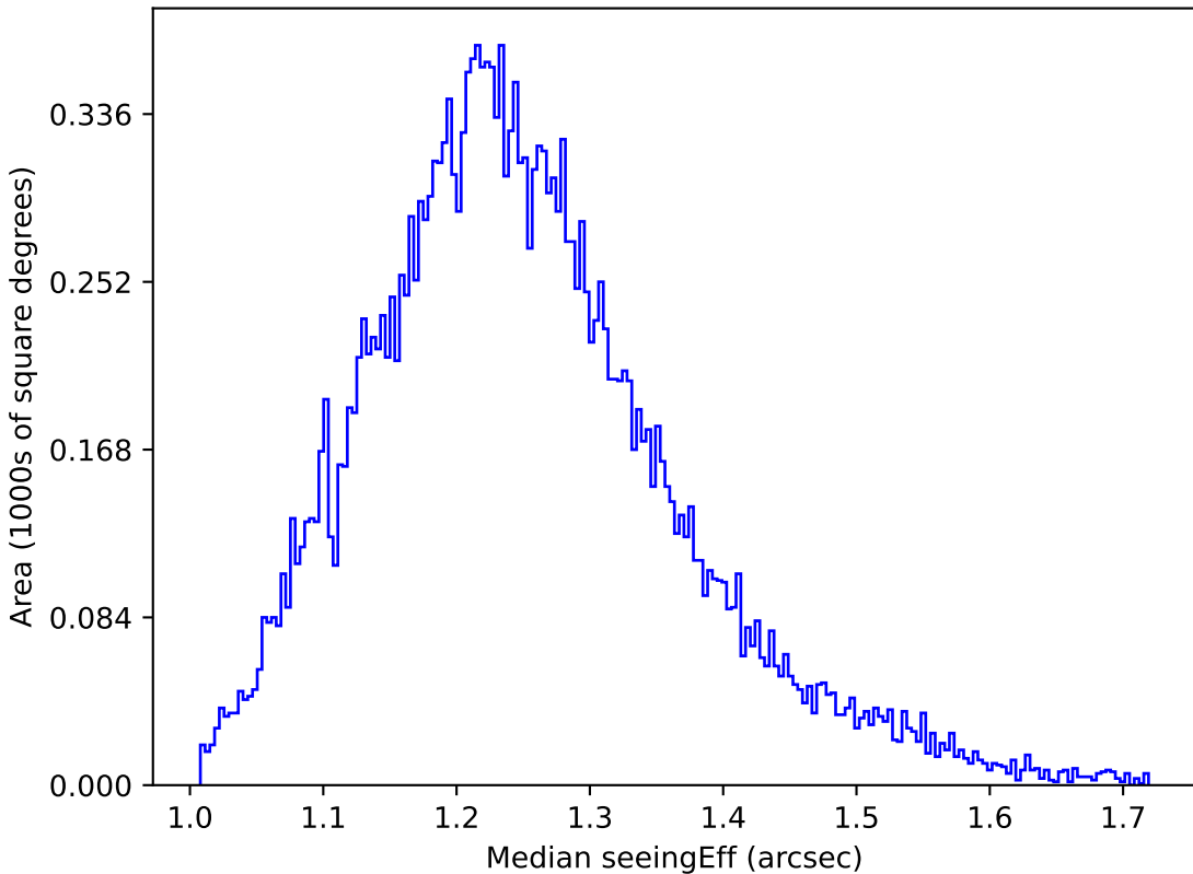
ddf_loaded_fl1_v3.4_10yrs All sky u band: Median seeingEff
