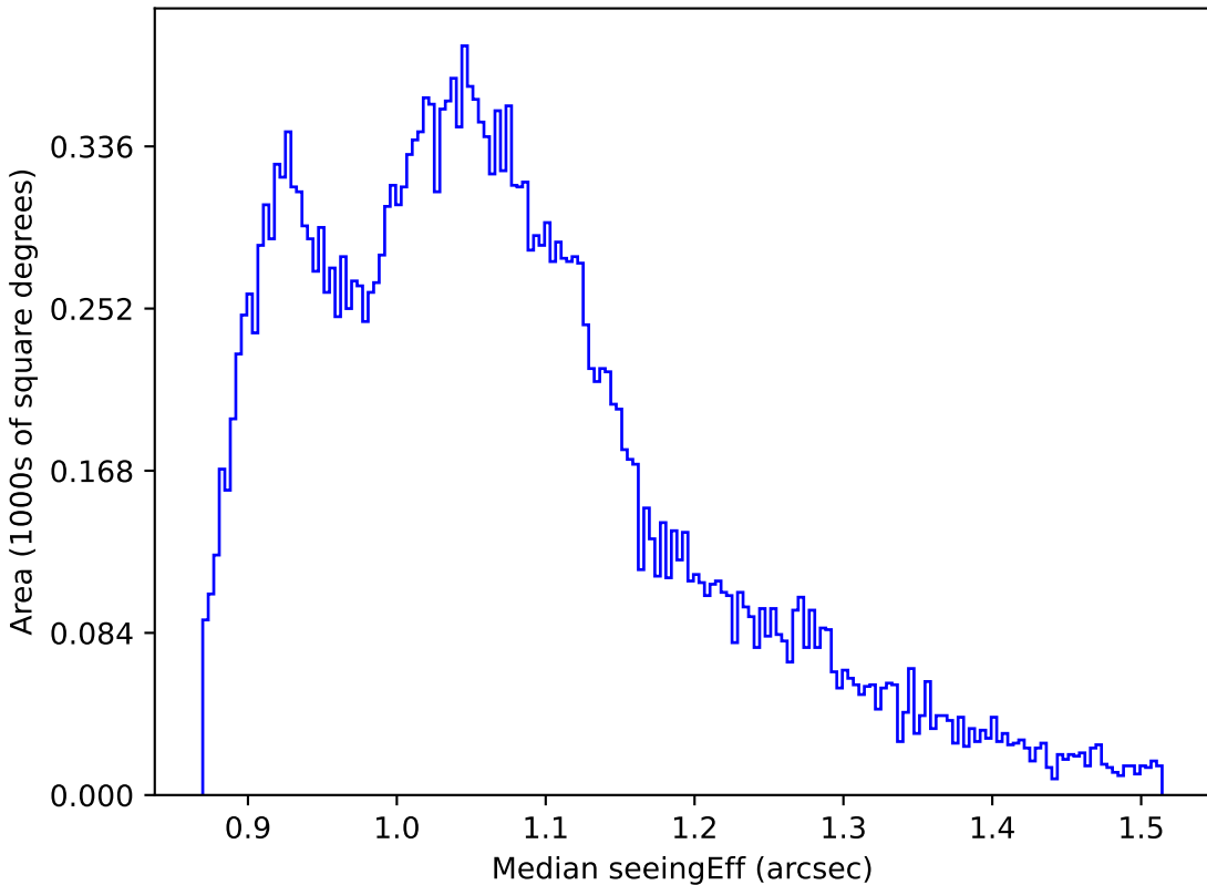
ddf_loaded_fl1_v3.4_10yrs All sky r band: Median seeingEff
