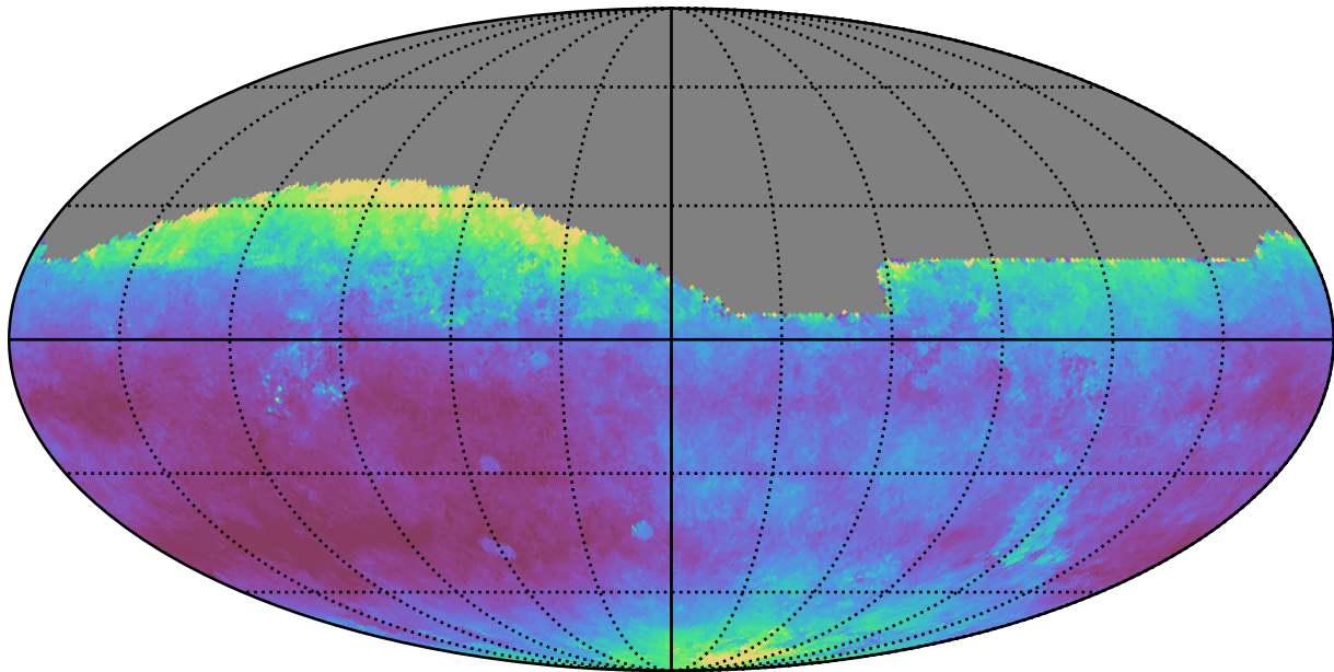
ddf_loaded_fl1_v3.4_10yrs All sky i band: Median seeingEff
