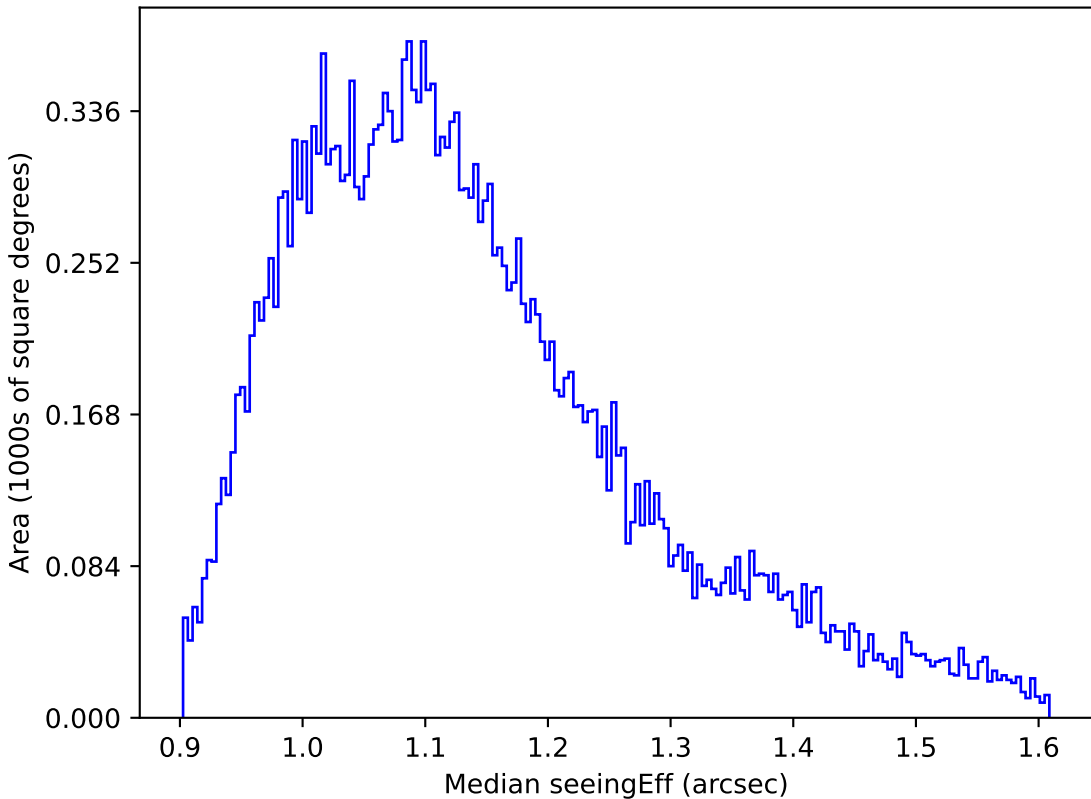
ddf_loaded_fl1_v3.4_10yrs All sky g band: Median seeingEff
