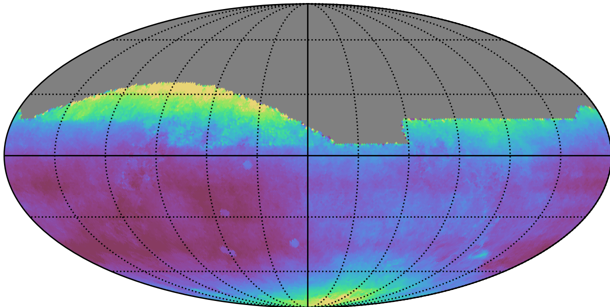
ddf_loaded_fl1_v3.4_10yrs All sky all bands: Median seeingEff
