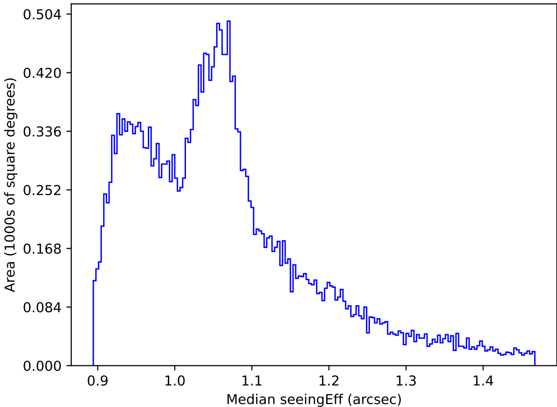
ddf_loaded_fl1_v3.4_10yrs All sky all bands: Median seeingEff
