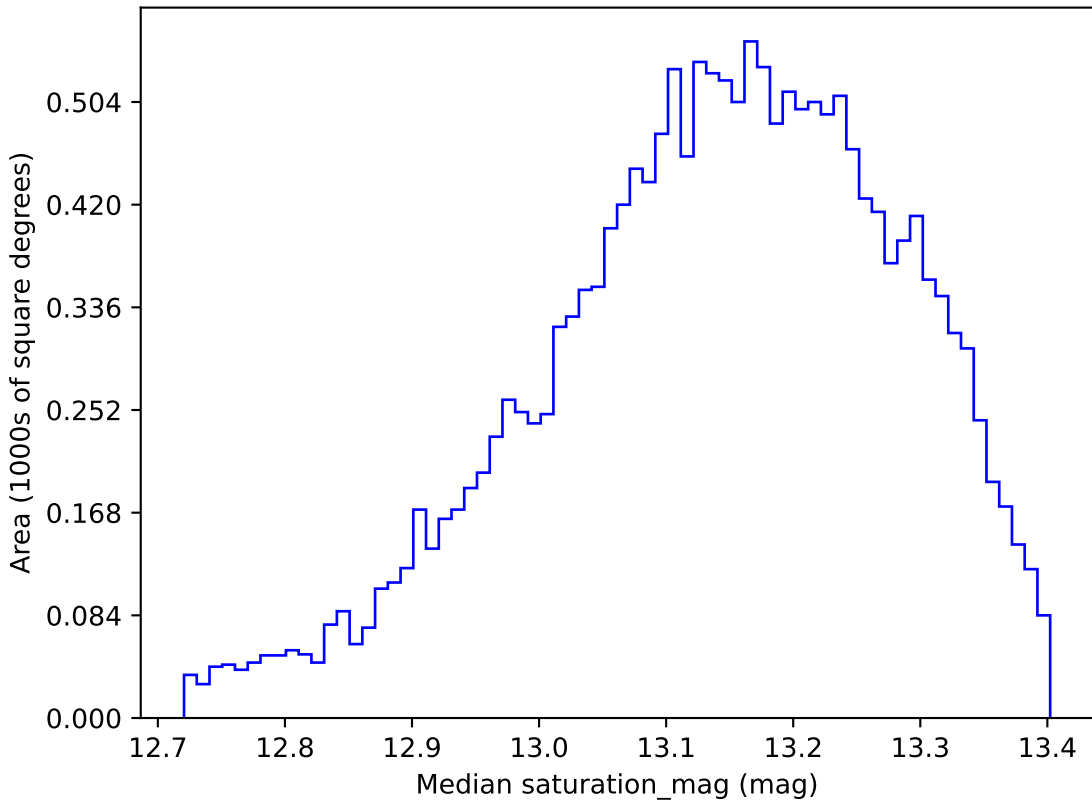
ddf_loaded_fl1_v3.4_10yrs WFD y band: Median saturation_mag
