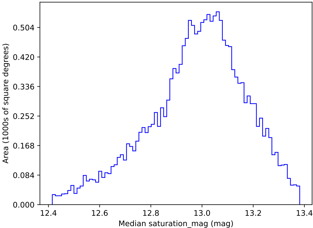
ddf_loaded_fl1_v3.4_10yrs WFD u band: Median saturation_mag
