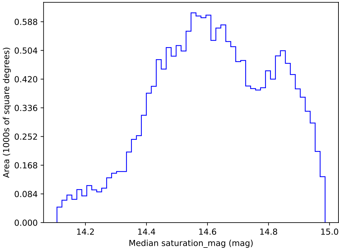
ddf_loaded_fl1_v3.4_10yrs WFD r band: Median saturation_mag
