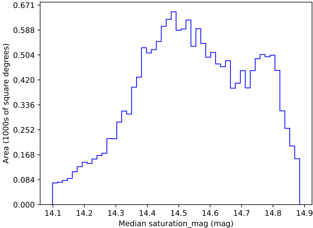
ddf_loaded_fl1_v3.4_10yrs WFD i band: Median saturation_mag
