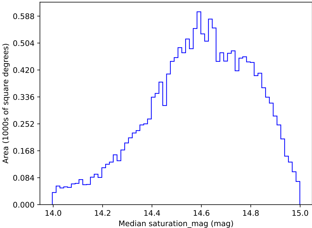
ddf_loaded_fl1_v3.4_10yrs WFD g band: Median saturation_mag
