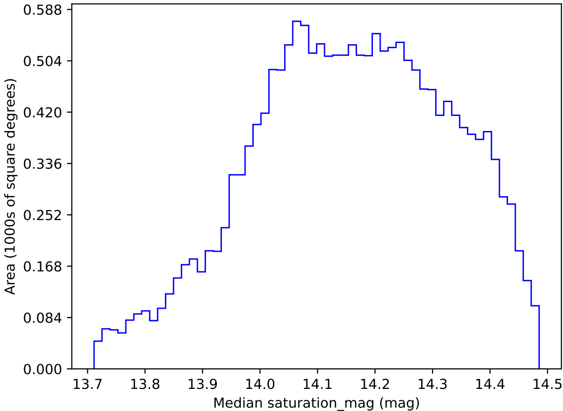
ddf_loaded_fl1_v3.4_10yrs WFD all bands: Median saturation_mag
