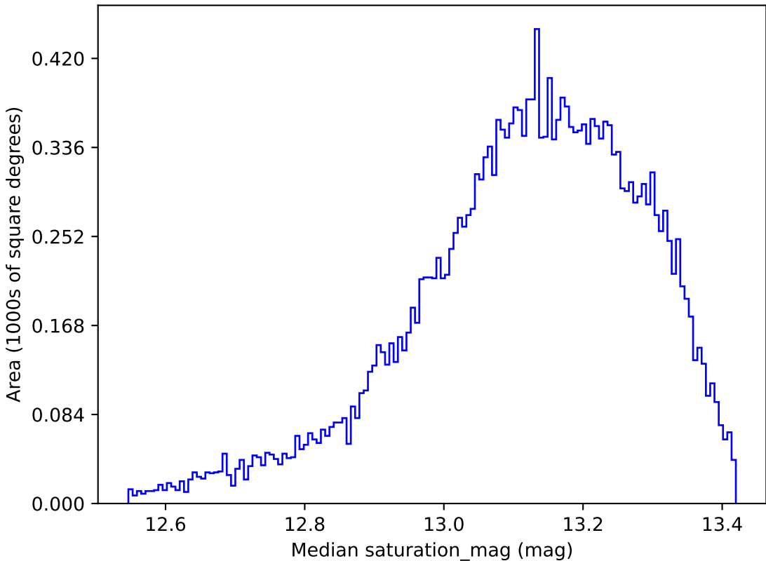
ddf_loaded_fl1_v3.4_10yrs All sky y band: Median saturation_mag
