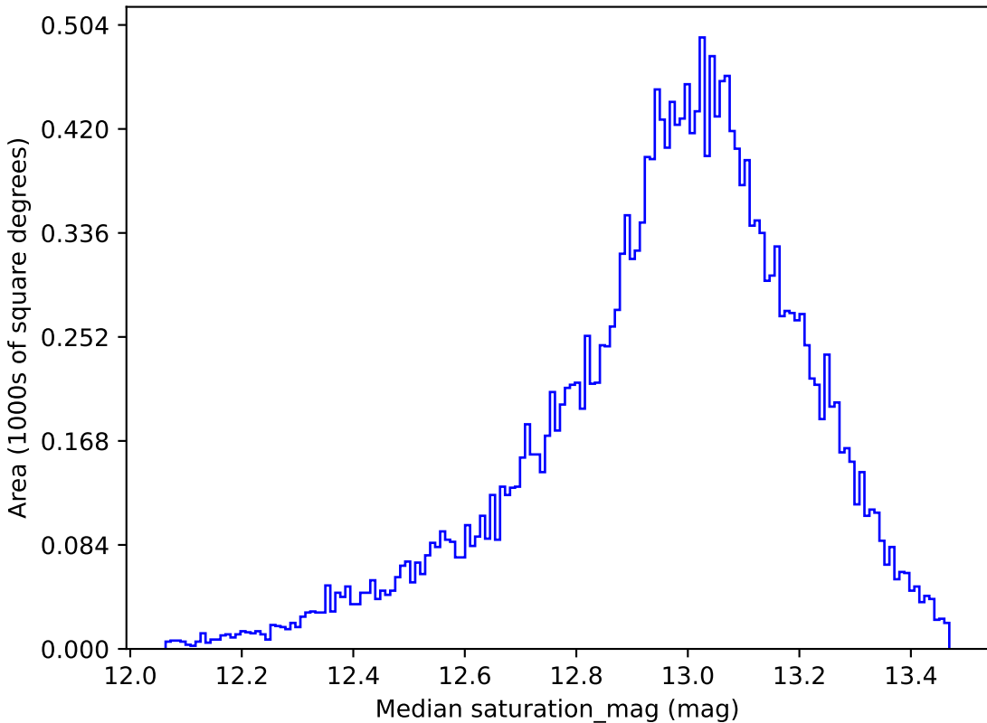
ddf_loaded_fl1_v3.4_10yrs All sky u band: Median saturation_mag
