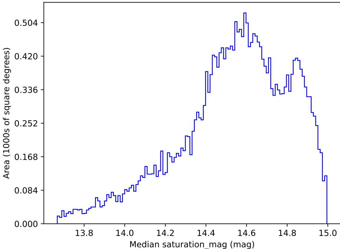
ddf_loaded_fl1_v3.4_10yrs All sky r band: Median saturation_mag
