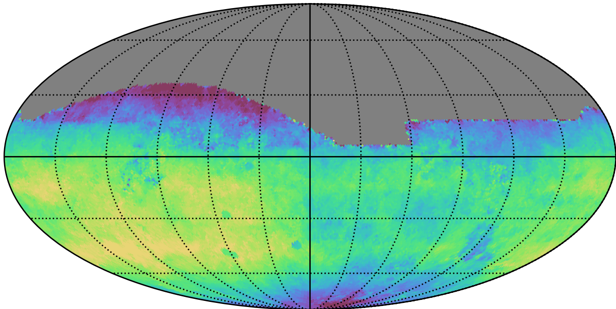
ddf_loaded_fl1_v3.4_10yrs All sky i band: Median saturation_mag
