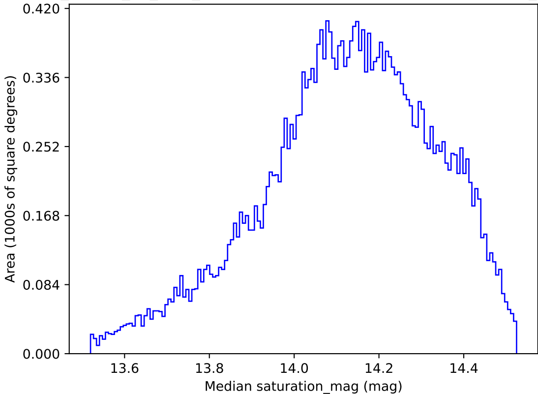
ddf_loaded_fl1_v3.4_10yrs All sky all bands: Median saturation_mag
