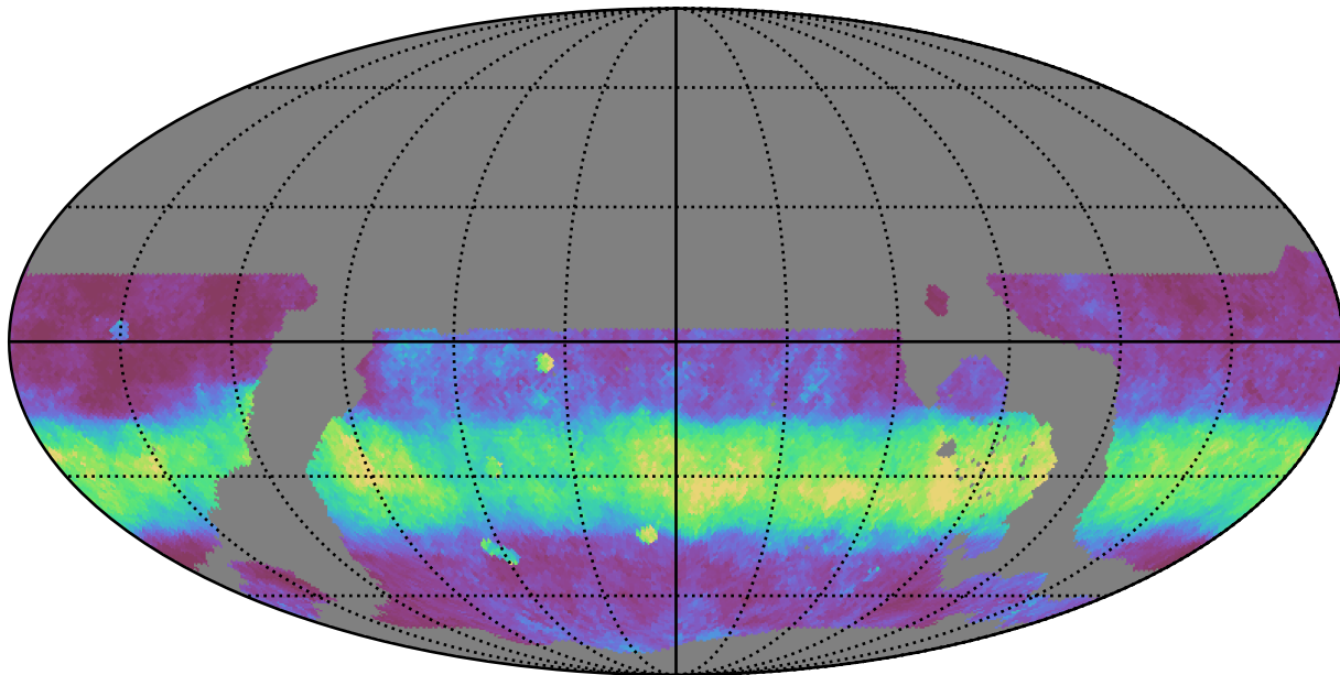
ddf_loaded_fl1_v3.4_10yrs WFD z band: Median normairmass
