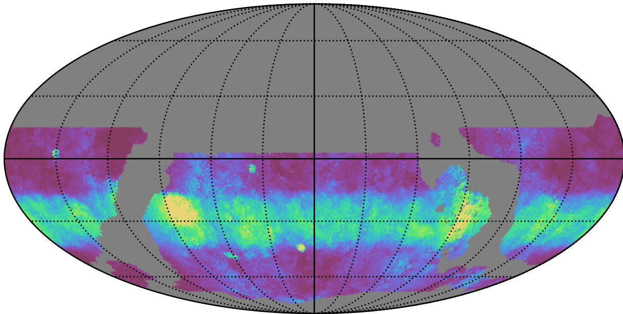
ddf_loaded_fl1_v3.4_10yrs WFD u band: Median normairmass
