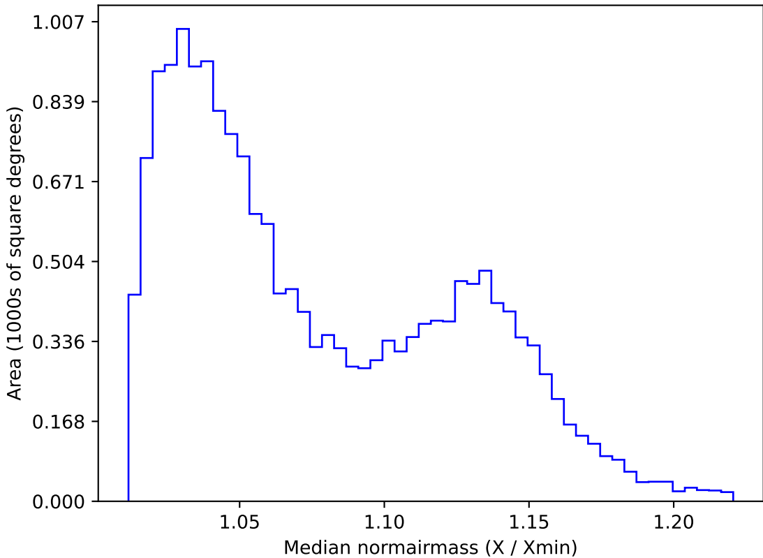
ddf_loaded_fl1_v3.4_10yrs WFD u band: Median normairmass
