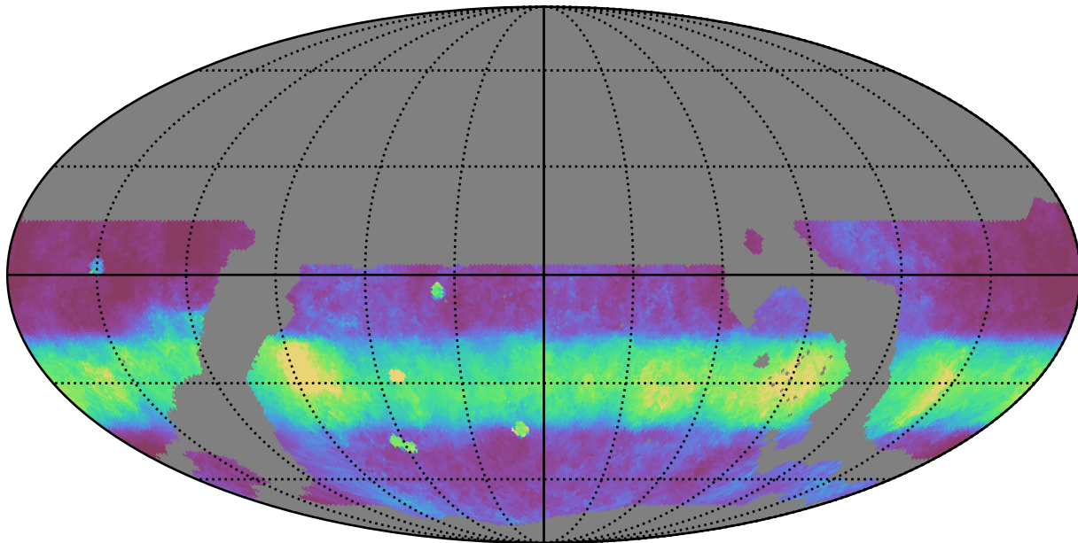
ddf_loaded_fl1_v3.4_10yrs WFD r band: Median normairmass
