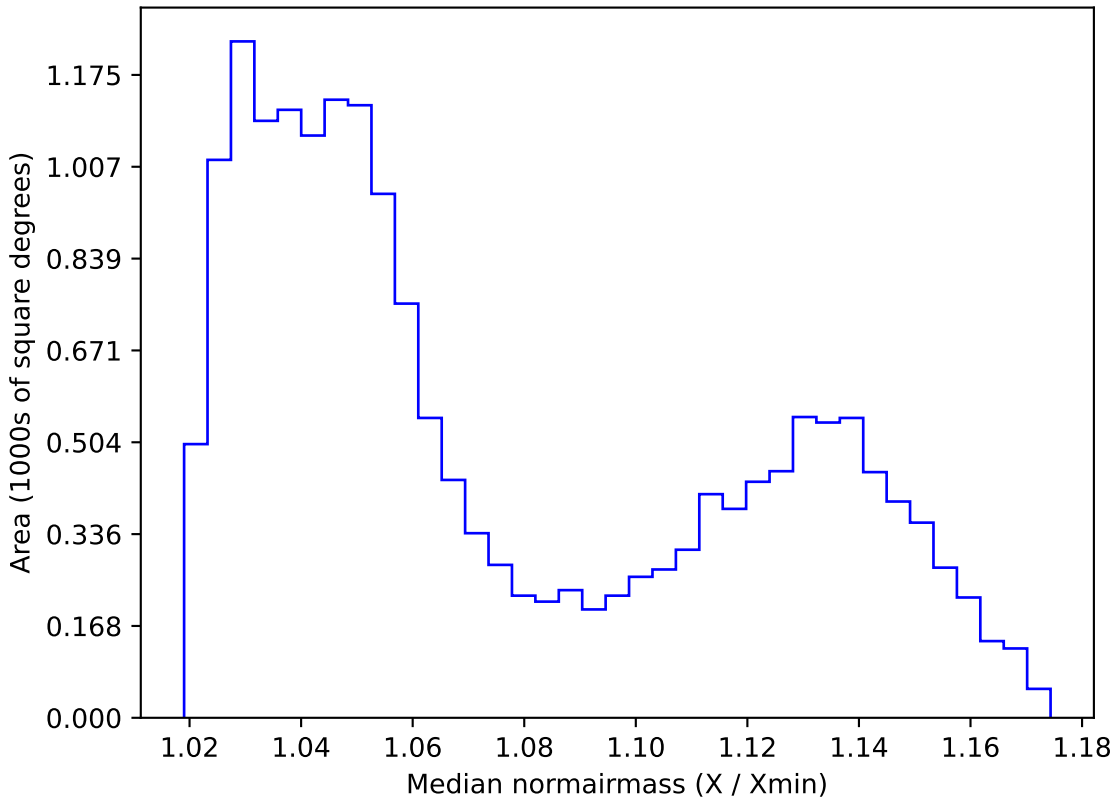
ddf_loaded_fl1_v3.4_10yrs WFD i band: Median normairmass
