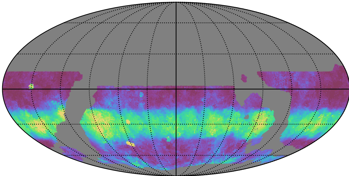
ddf_loaded_fl1_v3.4_10yrs WFD g band: Median normairmass
