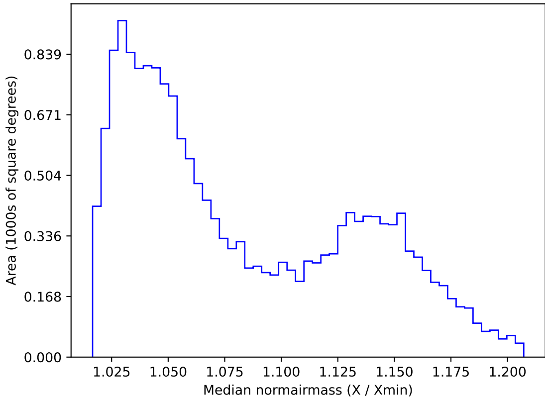
ddf_loaded_fl1_v3.4_10yrs WFD g band: Median normairmass
