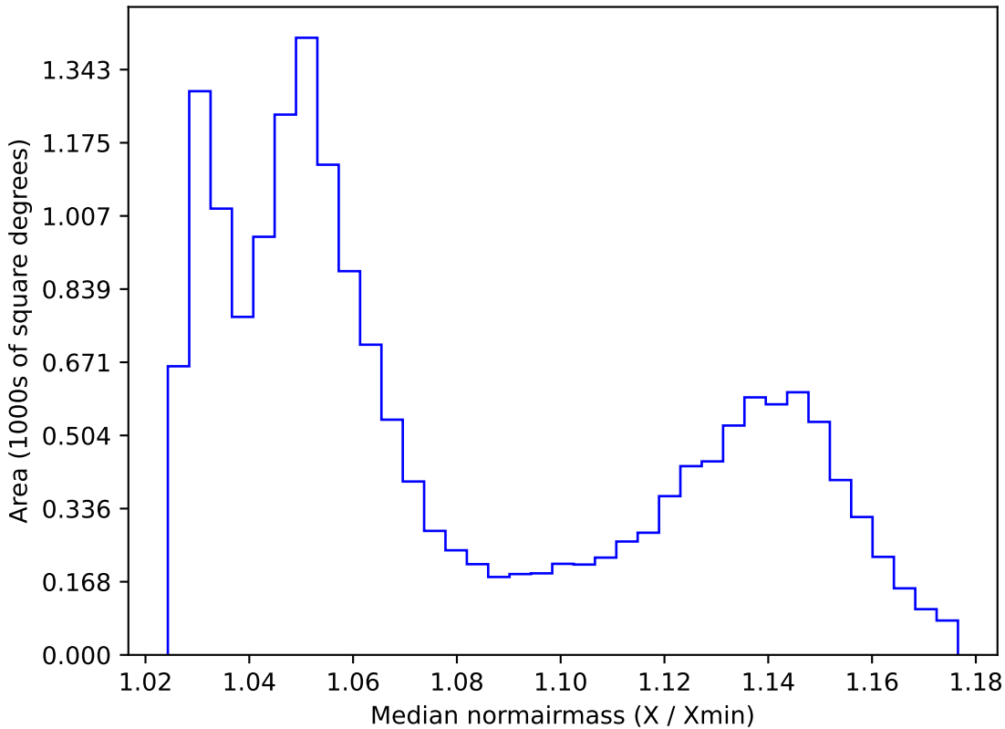
ddf_loaded_fl1_v3.4_10yrs WFD all bands: Median normairmass
